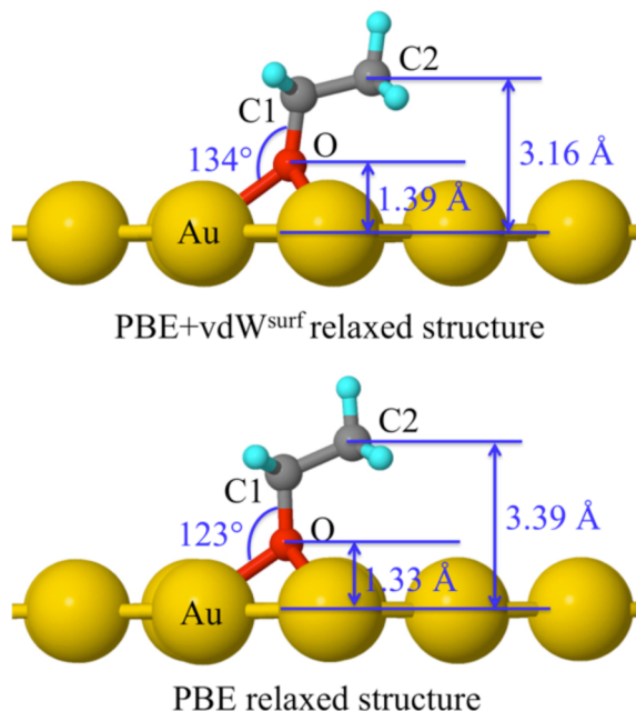
Figure 5. The structures of ethoxy (C 2 H 5 O) adsorbed on Au(111) with (top) and without (bottom) vdW interactions. Key bond lengths are changed by the vdW terms, including the Au-O, and Au-C 2 .
