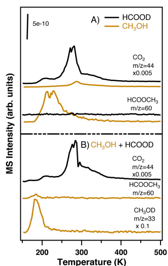
Figure 3: Temperature programmed reaction demonstrates the predominance of formate binding to the surface when CH 3 OH and HCOOH are co-adsorbed on O/Au(111) (O = 0.05 ± 0.01 ML) at 140 K. A) The characteristic reactions of formic acid (black) alone and pure methanol (gold). B) The products observed from dosing a mixture of the two. Products characteristic of formate decomposition (CO 2 ) predominate in the mixture. Exposures were controlled to dose ~0.5 ML of each reactant.
