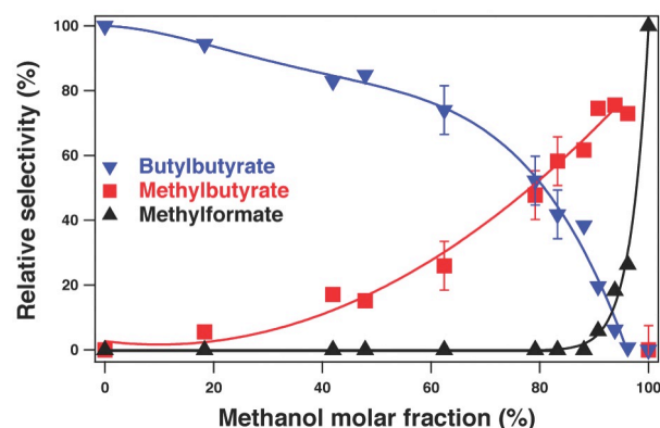
Figure 1: The selectivity for the esters formed from oxidative coupling of methanol and 1-butanol on O/Au(111) ( \theta_{\text{O}}=0.1 ML) depends strongly on the \text{CH}_3\text{OH}:\text{C}_4\text{H}_9\text{OH} due to the competition for reactive sites on the surface. Figure taken from ref. 2 with permission.
