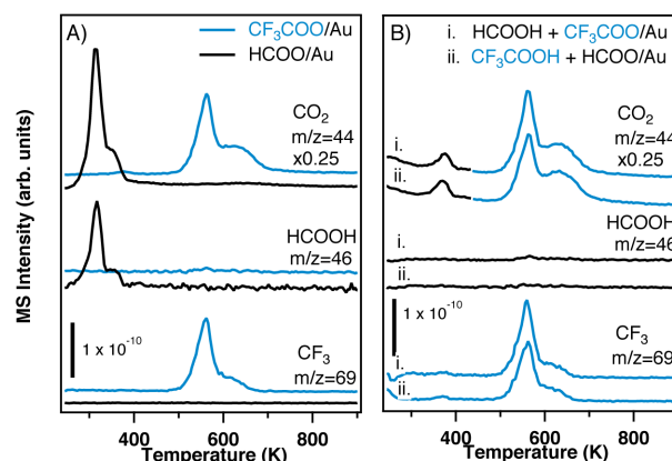
Figure 2. The displacement of formate by trifluoroacetic acid on Au(111) is demonstrated by monitoring characteristic decomposition reactions using temperature programmed reaction. (A) The characteristic “fingerprint” reaction products for reactions of the isolated formate (black) and trifluoroacetate (blue) yield different products and occur at very different temperatures. Formate decomposes to \text{CO}_2 and \text{HCOOH} at 300 K, whereas trifluoroacetate yields \text{CO}_2 and \text{CF}_3 at 580 K. (B) The exposure of adsorbed formate to excess trifluoroacetic acid yields products characteristic of adsorbed trifluoroacetate (at 580 K). The product amounts and temperatures are independent of the order of adsorption, clearly showing that trifluoroacetate binding is stronger.
